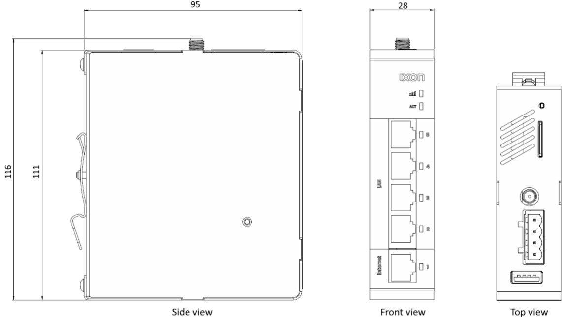
Figure 3: IXrouter3 dimensions
